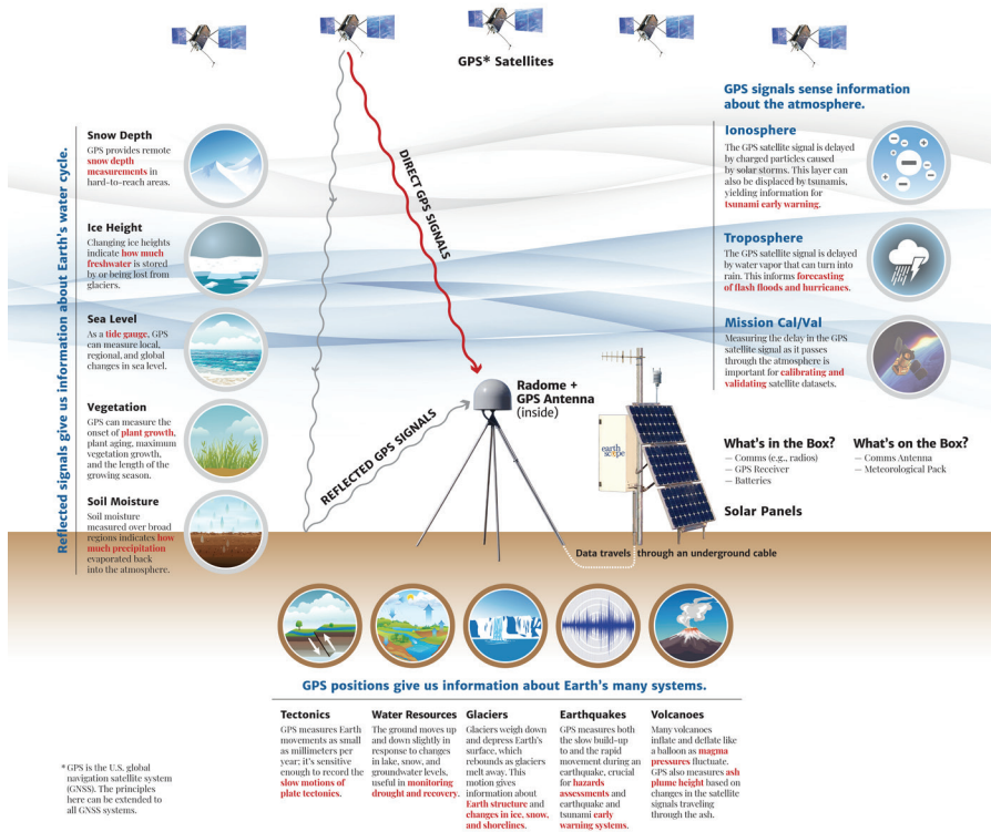
FIGURE 10.1.1 Ground-based GPS receivers play an important role in Earth science. GPS receivers precisely measure the latitude, longitude, and height of the receiver—information that is used for tectonic, volcano, and earthquake applications. Atmospheric researchers use the delays on the GPS signals to infer tropospheric water vapor and total electron content in the ionosphere. Reflected GPS signals can be used to measure soil moisture, snow depth, vegetation water content, and sea level. SOURCE: Courtesy of UNAVCO.
