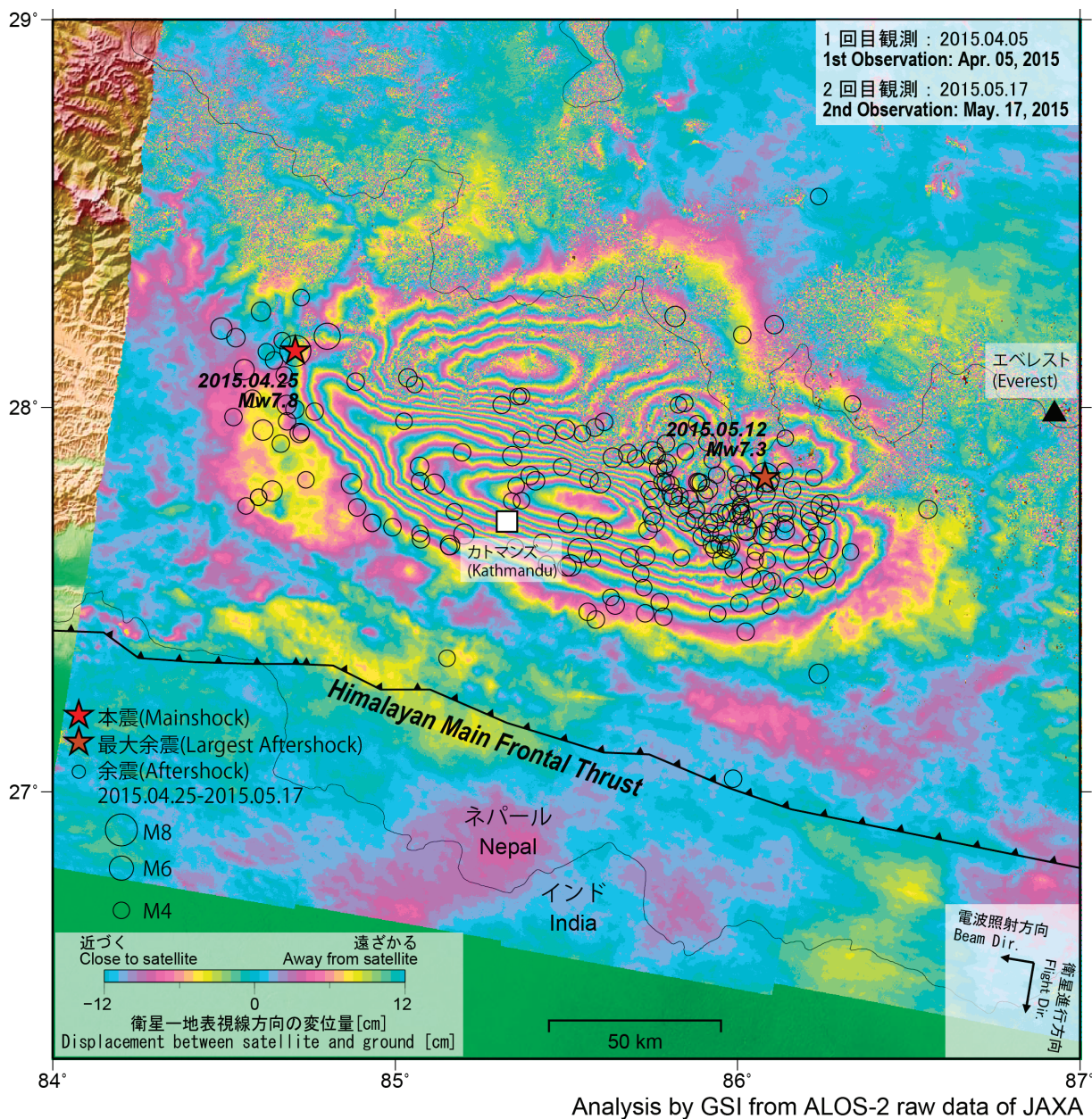
FIGURE 10.2 InSAR image of deformation for the Nepal M7.8 earthquake and M7.3 aftershock from Advanced Land Observing Satellite (ALOS)-2 interferometry. Repeated SAR acquisitions provide maps of ground displacement used to understand locations of possible large aftershocks and postseismic activity. This interferogram shows the benefits of using the longer wavelength SAR technology to be deployed in the NISAR mission for mapping line-of-sight ground displacement in a region of extreme topography. SOURCE: Geospatial Information Authority of Japan, "The 2015 Nepal Earthquake: Crustal Deformation Detected by ALOS-2 Data," last updated August 4, 2015, http://www.gsi.go.jp/cais/topic150429-index-e.html .
