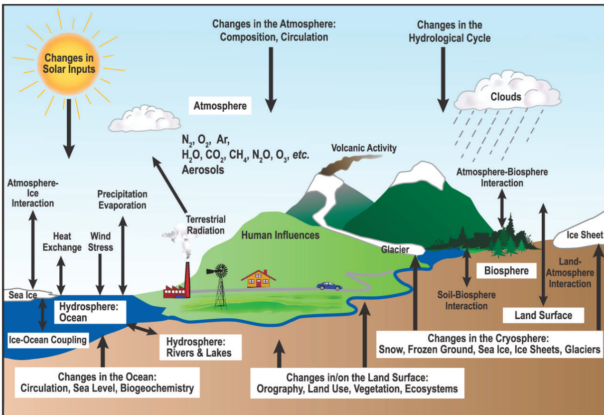
FIGURE 9.1 Schematic depicting components of the Earth system illustrating the coupled atmosphere, oceans, biosphere, and cryosphere system. Important processes such as changes in atmospheric composition owing to natural and human-influenced factors, and feedbacks such as those involving the hydrologic cycle (e.g., clouds), influence the state of the system—for example, land and ocean surface temperatures, precipitation, and sea level. SOURCE: IPCC (2007, p. 96).
